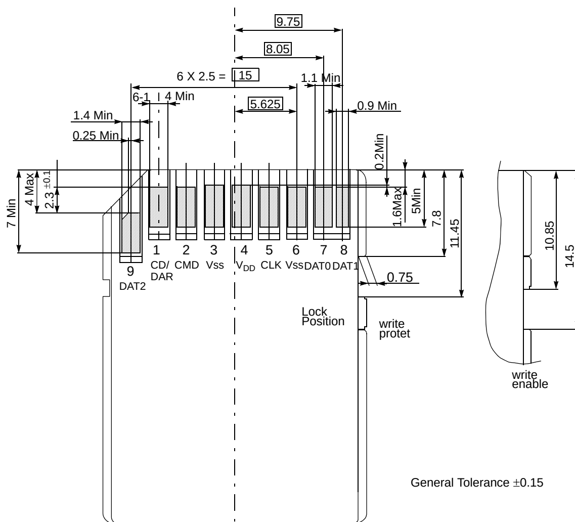
Figure 5-10. Mechanical Description: Bottom View
