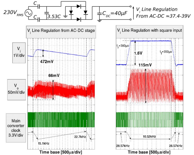
Figure 20.1.4: Line regulation response, while supplied by an example primary AC-DC converter as well as a 1.6V step-wise line variation.
