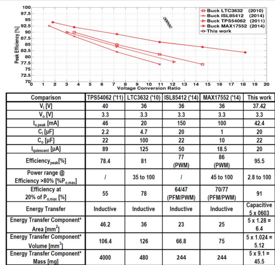
Figure 20.1.6: Performance summary and comparison.
