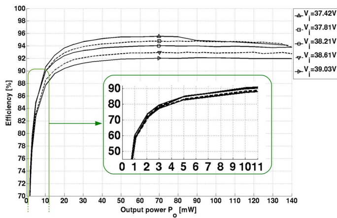
Figure 20.1.5: Efficiency versus load power for multiple input voltages, each corresponding to a theoretical maximum efficiency setting of 97% for V_i=37.42V down to 93% for an input voltage of 39.03V.
