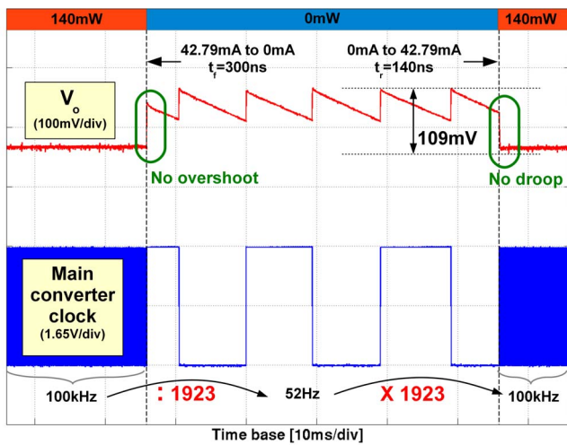
Figure 20.1.3: Load transient response of full load steps, while V_i=37.42V . The switching frequency changes instantly, allowing neither overshoot or undershoot to occur.
