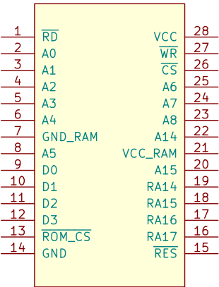
Figure D.14: MBC2 (Sharp SOP28-P-450) [8]
