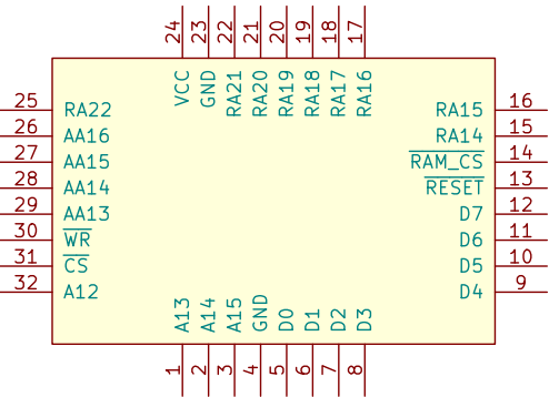
Figure D.15: MBC5 (Sharp QFP32-P-0707)
