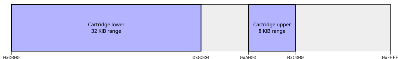
Figure 12.5: Cartridge address space areas
